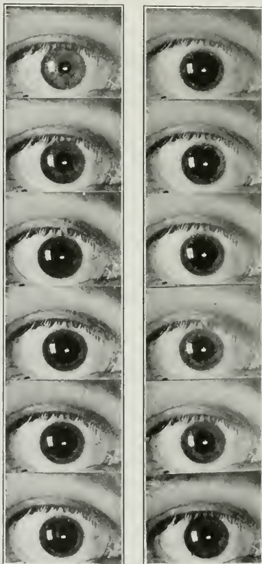
Fig. 7. Iris Opening and Closing.
